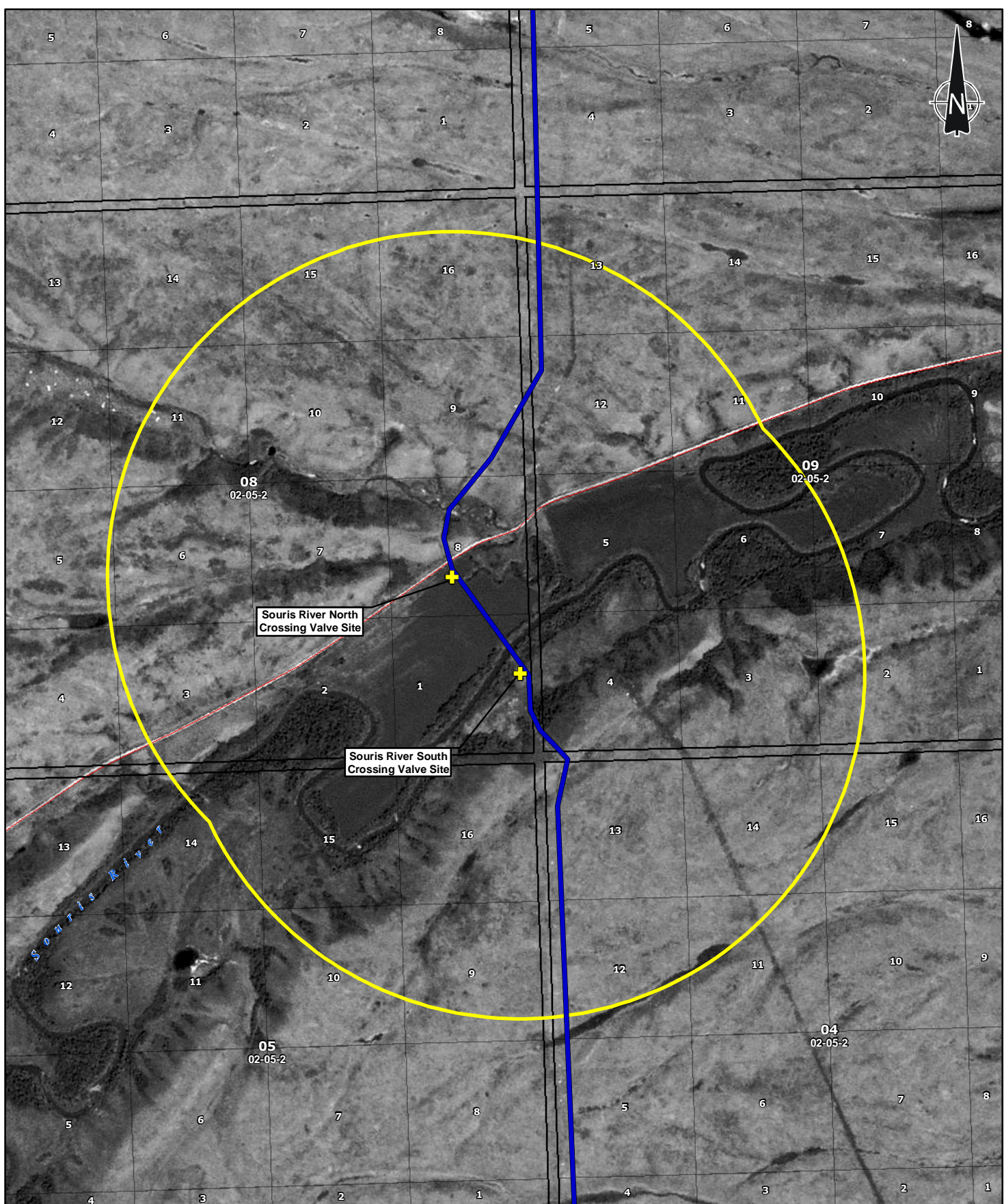
FIGURE 2B AERIAL VIEW OF THE EXISTING VALVE SITES AT THE SOURIS RIVER
